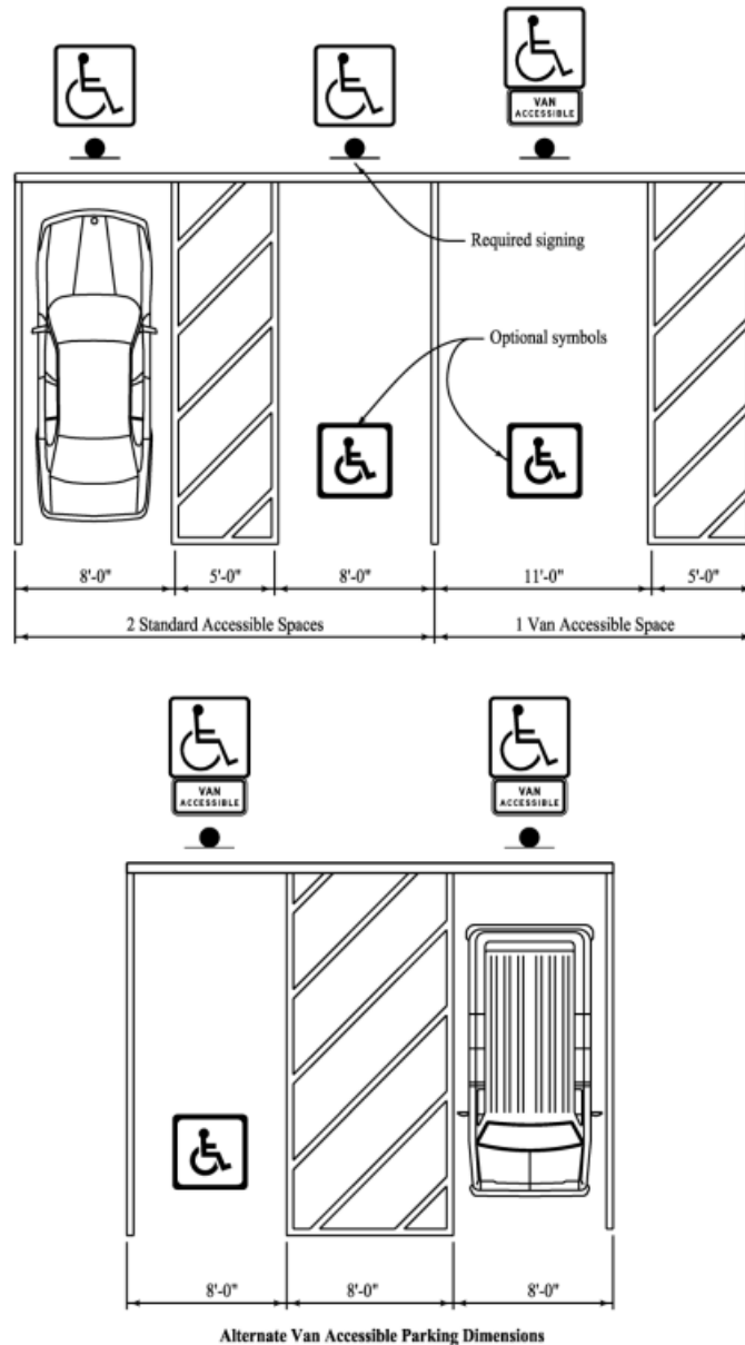
Figure 8B-1.02: Accessible Space Dimensions
